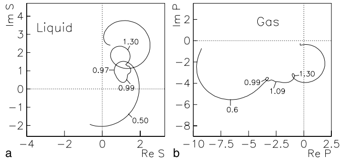
Fig. 6. Argand diagrams for the \pi\pi S -wave of [5] for a ^1S_0 annihilation, b ^3P_1
